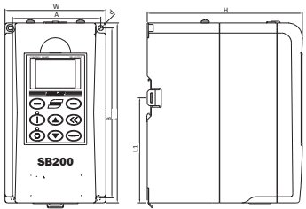
Outline Drawing of the SB200 Series (SB200-1.5T4—5.5T4) (Installable with a standard DIN Guide Rail)
